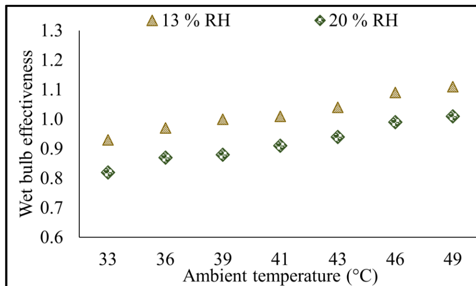
Figure 11. Wet bulb effectiveness at V=6.1\text{ m/s} and T_w = 20^\circ\text{C}
