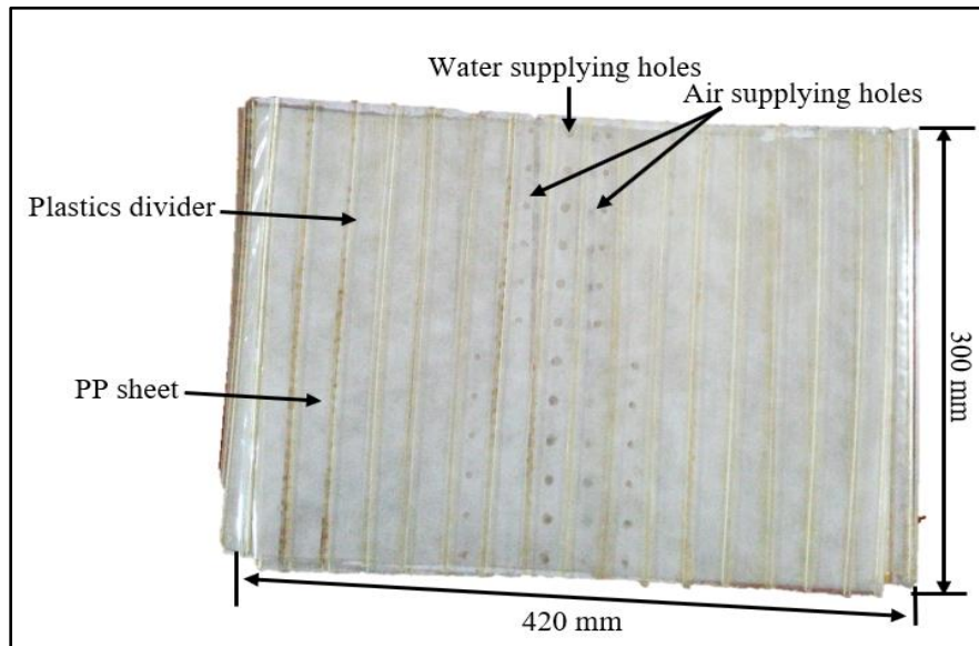
Figure 4. Dry channel of the HMX
