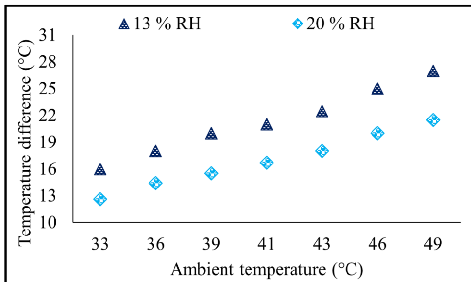
Figure 9. Temperature drops in dry channels at V=6.1\text{m/s} and T_w = 20^\circ\text{C}
