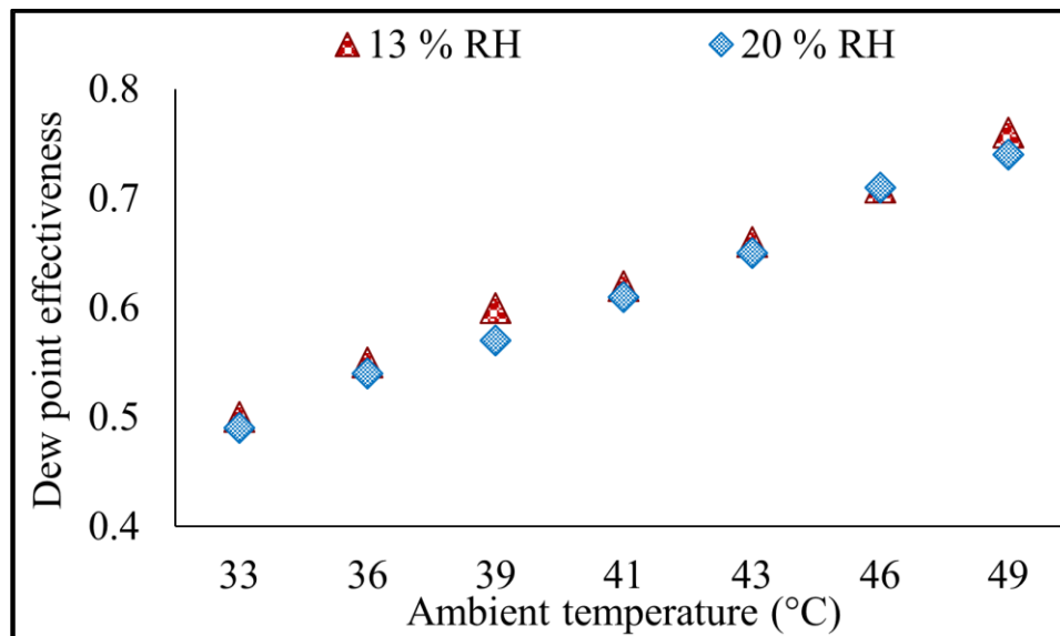
Figure 10. Dewpoint effectiveness at V=6.1\text{m/s} & T_w = 20^\circ\text{C}
