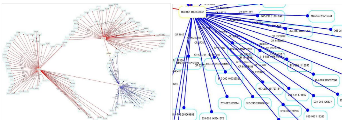
Figure 1 : graph database
