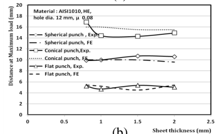
Fig. 15. Comparison between experimental and FE results of (a) Maximum load vs. sheet thickness and (b) Distance at maximum load vs. sheet thickness for different punch shapes.
