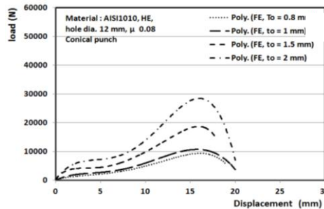
Fig. 3. An example of the FE-predicted Load /displacement curves for different sheet thickness, \mu = 0.08 , \phi_{\text{hole}} = 12 mm and conical punch geometry
