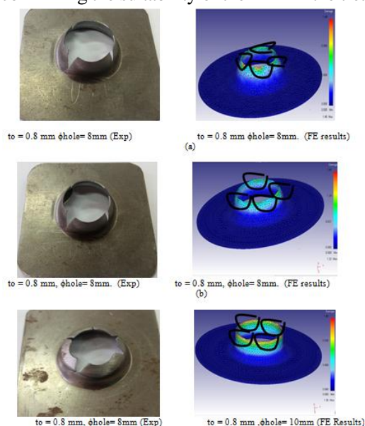
Fig. 16. Comparison between experimentally-obtained fractures (left) and FE- predicted damage sites (right) using different punch shapes
