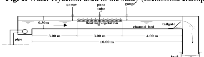
Fig. 2. Experimental flume.
