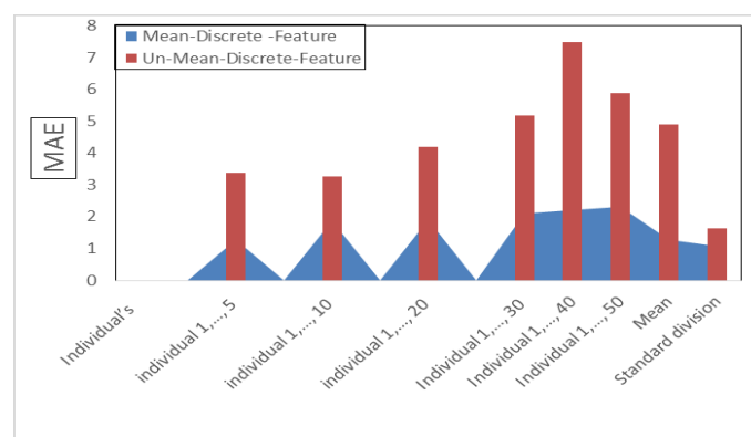
Fig. 3 - Uni-representation (Mean-Discrete) comparison for intra-class.
