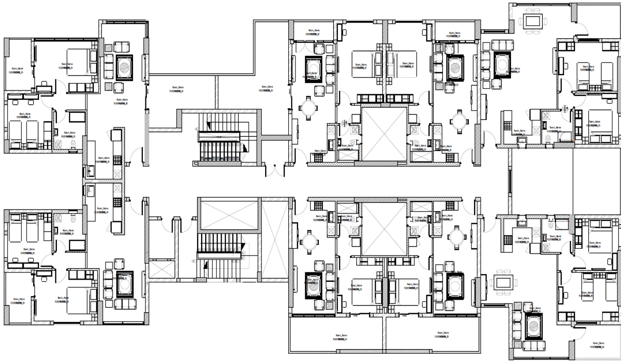
Fig. 5: R3 district, type OC building floor plan
