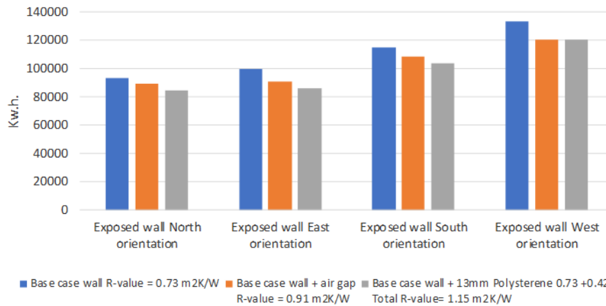
Fig. 6: Annual energy consumption of the case study building in R3 new capital- Type OC building after improving the building envelope
