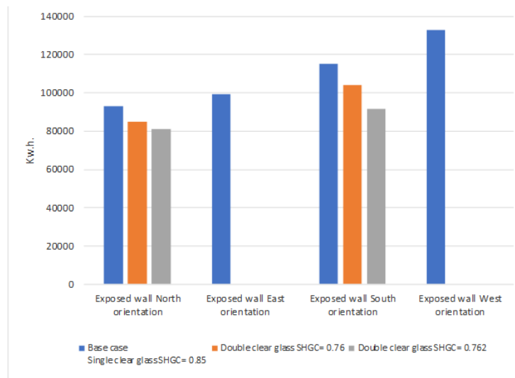
Fig. 7: Required SHGC for openings in elevations with WWR more than 30% in Cairo and delta climatic zone Source: Researchers using Design Builder Software
