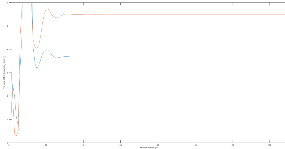
Fig. 3.3: The graph of a solution of system (3.4.2) with A = 3 and B = 4
