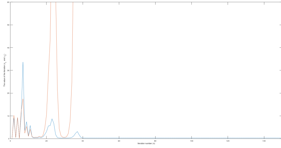
Fig. 3.1: The graph of a solution of system (3.4.1) with A = 0.3 and B = 0.5
