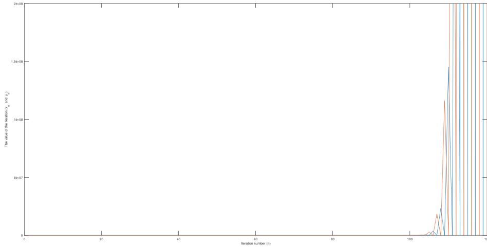
Fig. 2.1: The graph of a solution of system (2.5.1) with A = 0.2 and B = 0.8
