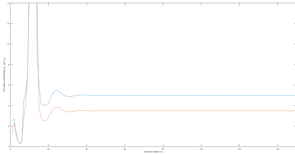
Fig. 2.2: The graph of a solution of system (2.5.1) with A = 4 and B = 2.5
