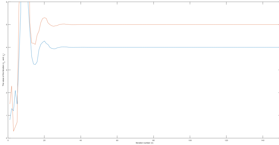
Fig. 2.3: The graph of a solution of system (2.5.2) with A = 3 and B = 4
