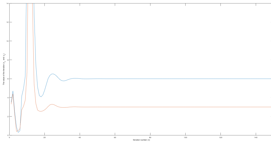
Fig. 3.2: The graph of a solution of system (3.4.1) with A = 4 and B = 2.5
