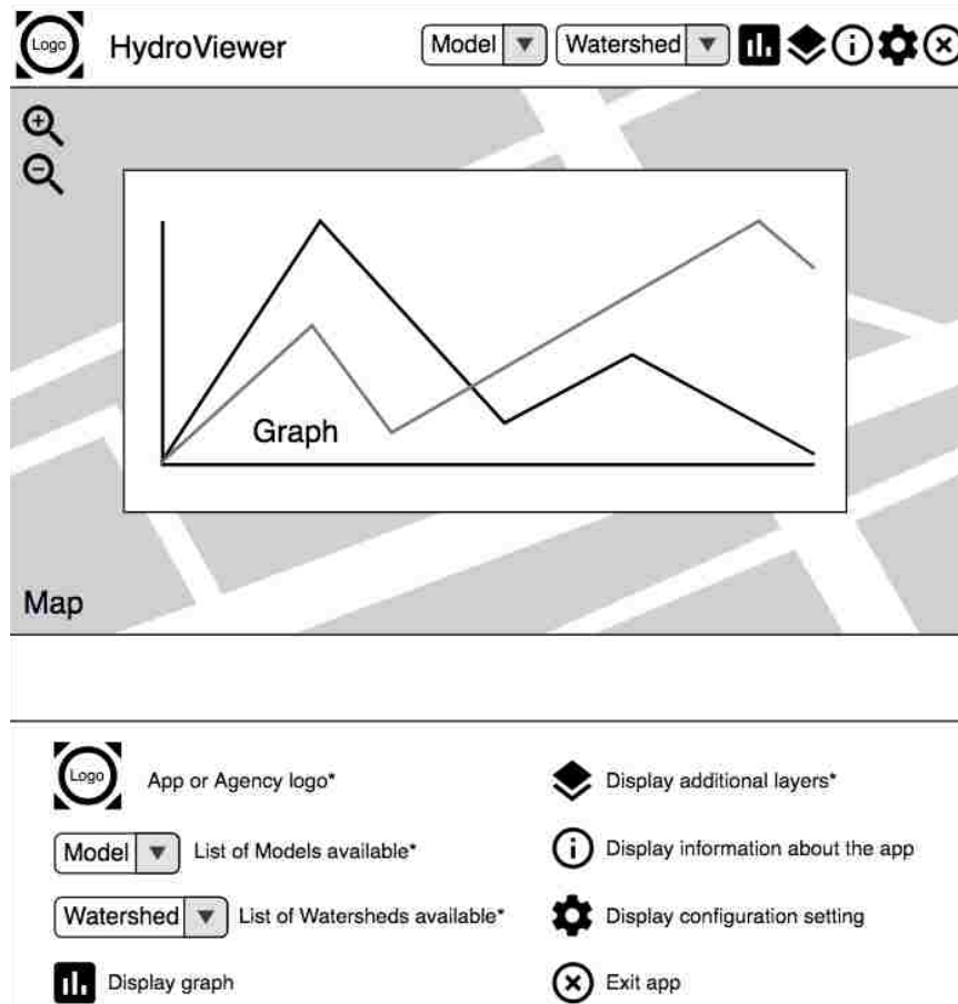
Figure 4-4. HydroViewer app design.
