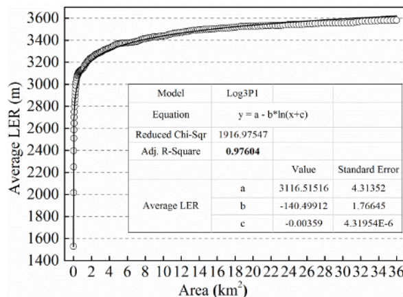
Figure 1 Fitted curve for the relationship between different grid units and local elevation range (LER) in China.
