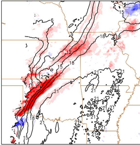
Figure 17. Composite differences (shaded) and full-ensemble-mean (contoured) of (a) 925 hPa dew point temperature (°C) and surface to 850 hPa average water vapor mixing ratio (g kg -1 ) at 2200 UTC 31 May 2013.
