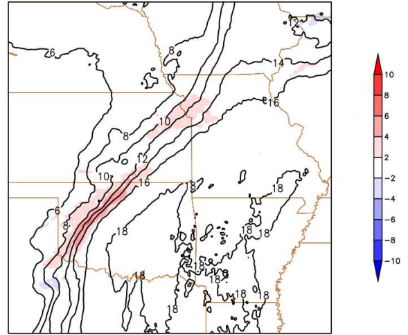
Figure 17. Composite differences (shaded) and full-ensemble-mean (contoured) of (a) 925 hPa dew point temperature (°C) and surface to 850 hPa average water vapor mixing ratio (g kg -1 ) at 2200 UTC 31 May 2013.
