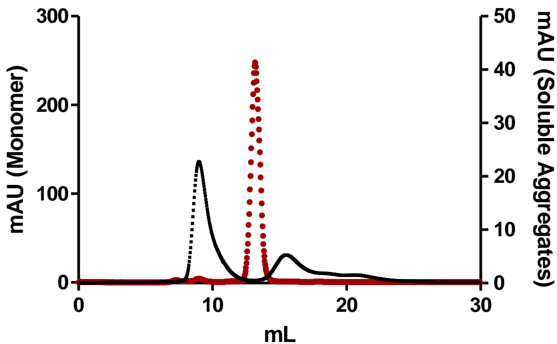
Figure 2.1. FPLC-SEC purification profile for Aβ 1-40 monomer (red) and Aβ 1-40 soluble aggregates (black). The FPLC utilizing SEC elutes large aggregates within the void volume followed by smaller monomer species of Aβ 1-40 within the included volume.
