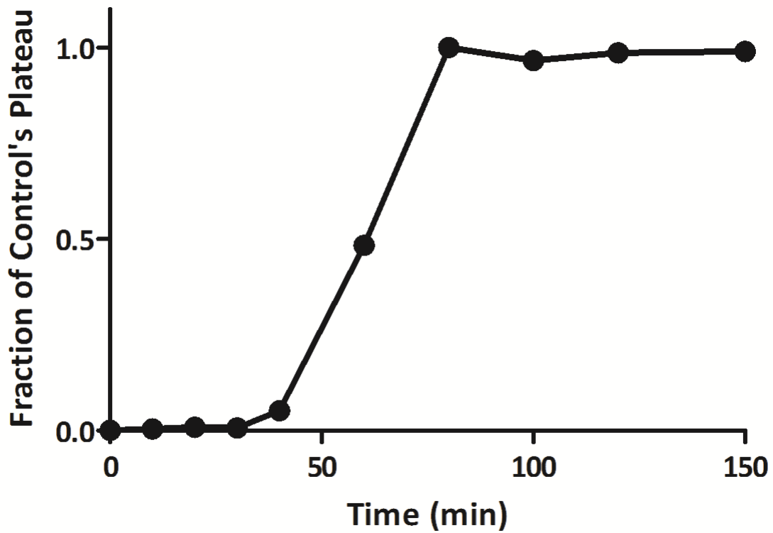
Figure 3.1. A \beta 1-40 monomer aggregation. A \beta 1-40 monomer aggregation exhibits three stages: the lag period, a rate limiting step where oligomerization occurs; the growth phase, a period of soluble aggregate growth through elongation and association into fA \beta ; and a plateau phase, where insoluble fA \beta , soluble aggregates, and oligomers are in equilibrium.
