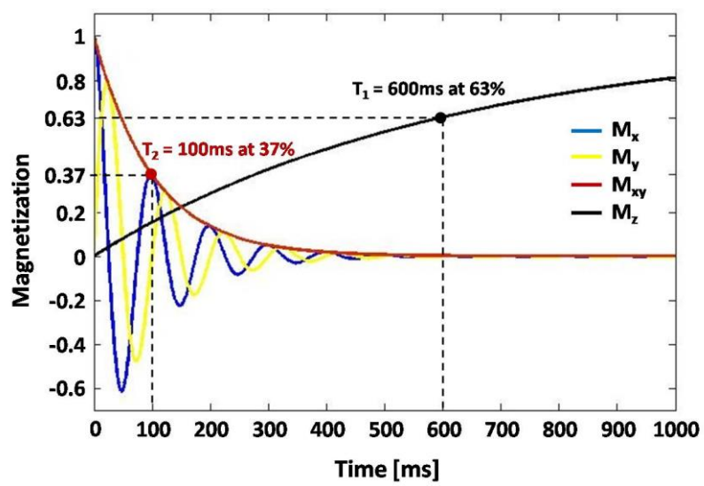
Figure 2.2. Free induction decay, T_1 and T_2 relaxation time.
