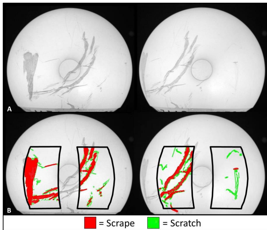
Figure 24: Scratch and scrape identification. (a) Diffused-light images of a femoral head displaying both scratch and scrape damage, captured from two orientation directions 30^\circ apart circumferentially. (b) Image processed results characterizing regions of damage. The sectors outlined in black indicate regions of interest analyzed for this particular image. (The top of the femoral head was captured and analyzed in companion polar images.)
